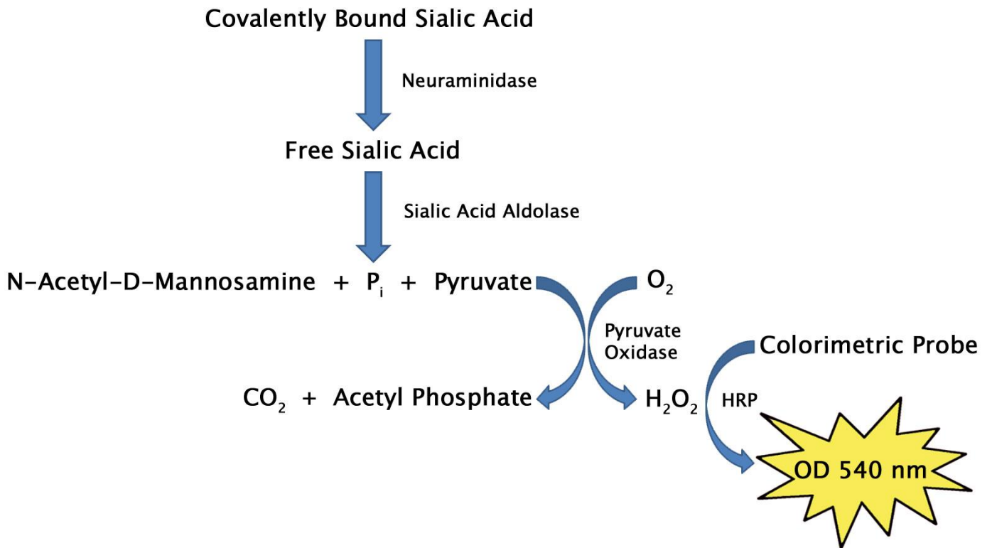
Figure 1. Sialic Acid Assay Principle.
