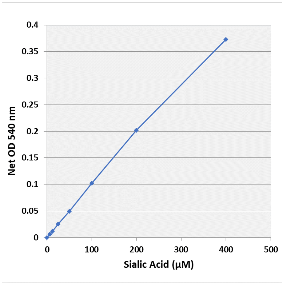
Figure 2: Sialic Acid Standard Curve.
